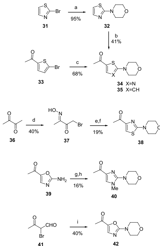
Scheme 3. Reagents and conditions: (a) morpholine, sealed tube, 100 °C, 3 d; (b) n -BuLi, THF, −78 °C; Ac 2 O, −60 °C, 1 h; (c) morpholine, sealed tube 145 °C; (d) Br 2 , hydroxylamine hydrochloride, Na 2 CO 3 , H 2 O; (e) morpholine-4-carboxylic acid amide, EtOH, reflux, 2 h, 99%; (f) H 2 SO 4 , EtOH, NaNO 2 , 50 °C, 2 h, 19%; (g) morpholine, H 2 O, reflux, 33%; (h) NaH, MeI, THF, rt, 1.5 h, 49%; (i) morpholine-4-carboxylic acid amide, acetone, rt, 1 h; reflux, 1 h.
