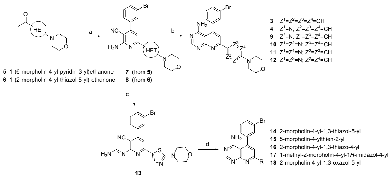
Scheme 1. Reagents and conditions: (a) 2-(3-bromobenzylidene)malononitrile, NH 4 OAc, DCE, reflux; (b) formamide, 180 °C; (c) CH(OEt) 3 , NH 4 SO 4 , reflux; NH 3 , EtOH, rt; (d) o -DCB, reflux.
